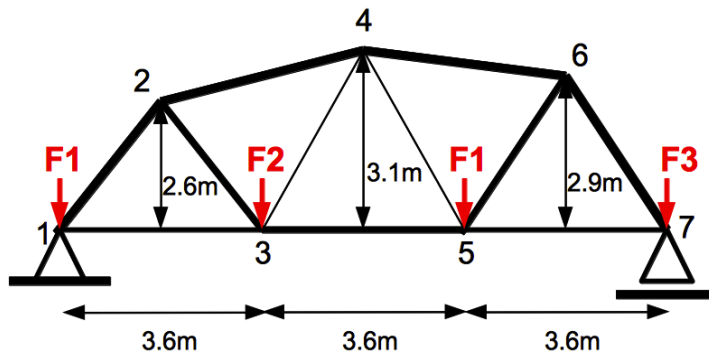
Figure 5: Best design of the 2D truss problem. Thicker lines symbolize truss members with larger cross sectional areas. The largest deflection is in vertical direction at node 7.
