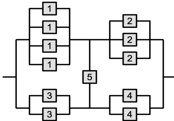
Figure 7: Best reliability-redundancy allocation for the bridge system. Redundancy has been added at components 1, 2, 3, and 4.
