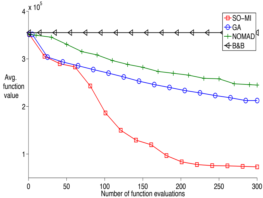
Figure 4: Objective function value for feasible points averaged over 30 trials vs. number of function evaluations; test problem 18, truss dome design optimization, minimization problem
