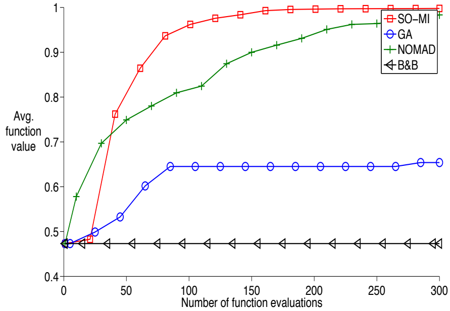
Figure 6: Objective function value for feasible points averaged over 30 trials vs. number of function evaluations; test problem 21, reliability-redundancy allocation for series-parallel configuration, maximization problem
