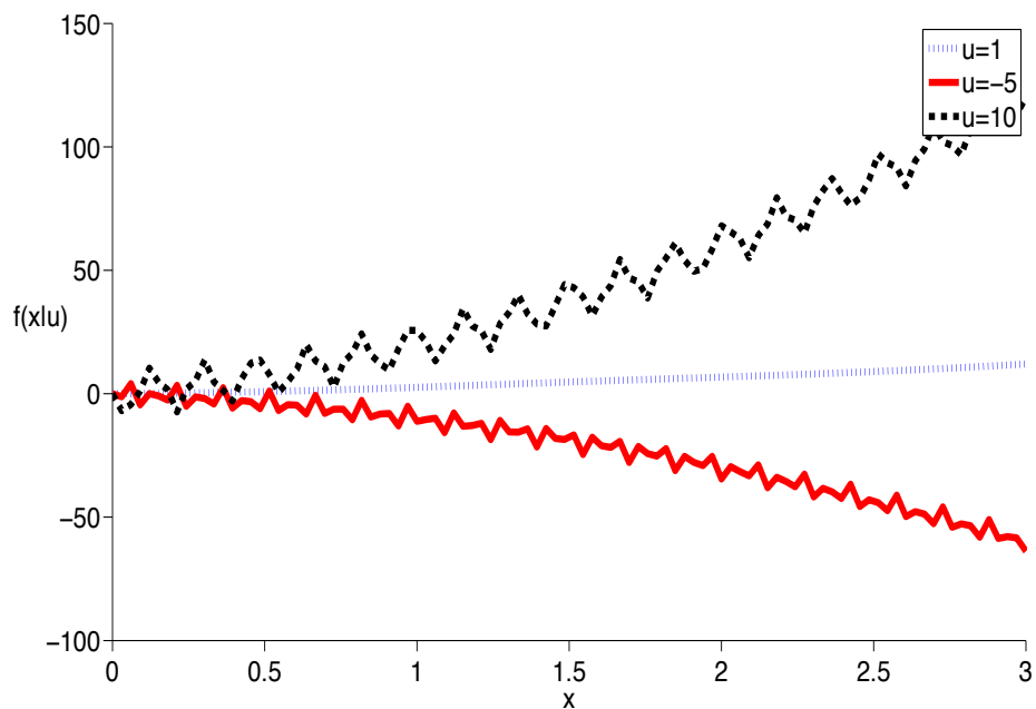
Figure 1: Illustrated is the function f(x, u) = ux + u \sin^3(u^3x) + ux^2 for three different fixed values of u . The function may be multimodal depending on the discrete variable values.
