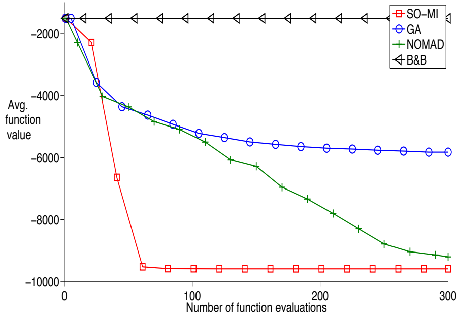
Figure 2: Objective function value for feasible points averaged over 30 trials vs. number of function evaluations; test problem 12, box-constrained minimization problem
