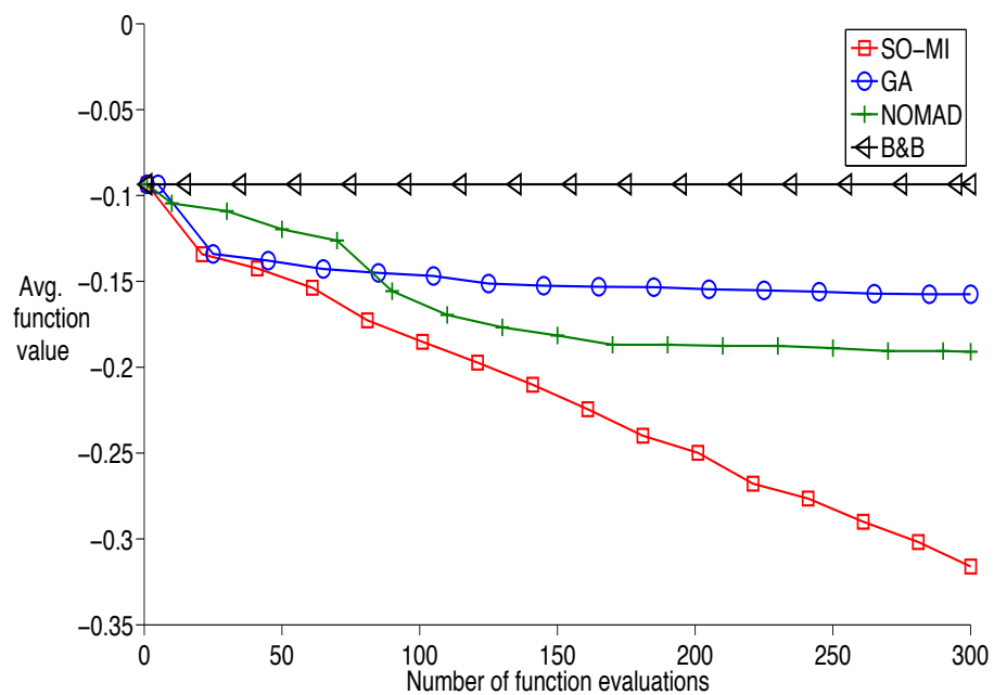
Figure 3: Objective function value for feasible points averaged over 30 trials vs. number of function evaluations; test problem 5, constrained minimization problem
