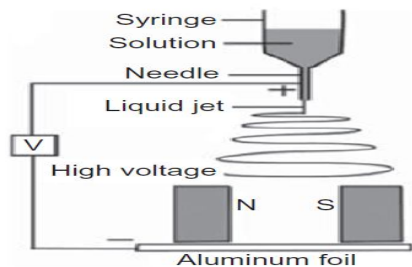
Figure 4. Magnetic electrospinning.
