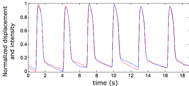
FIGURE 3. A representative displacement measurement showing overlaid CaPIV (blue) with fluorescence and PIV (shown in red) without fluorescence.
