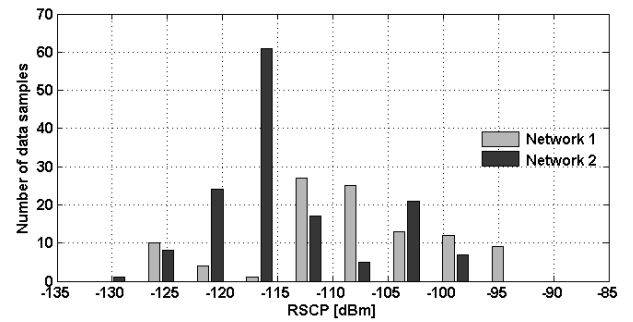
Fig. 5. Scenario 1: the received power levels of two different networks.
