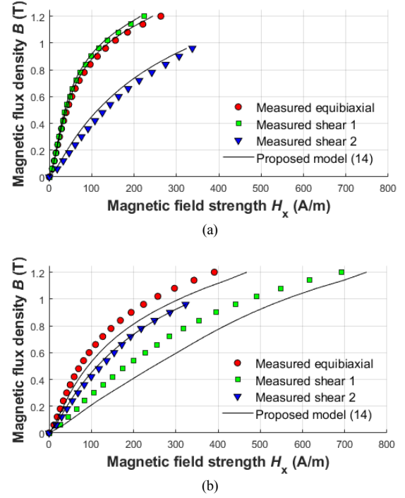
Fig. 3. Comparison of the B(H_x) curves obtained from the equivalent stress model (14) to those measured with the single-sheet tester under multiaxial loadings (3) when (a) \sigma = 20 MPa and (b) \sigma = -20 MPa.
