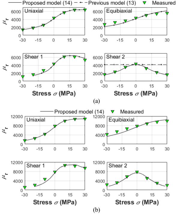
Fig. 2. Comparison of the measured relative permeabilities under multiaxial stresses to those interpolated from uniaxial measurements using the proposed equivalent stress model (14) and the previous model (13) (a) at B = 1 T and (b) B = 0.5 T. In (a) the results with the previous model (13) are also shown.
