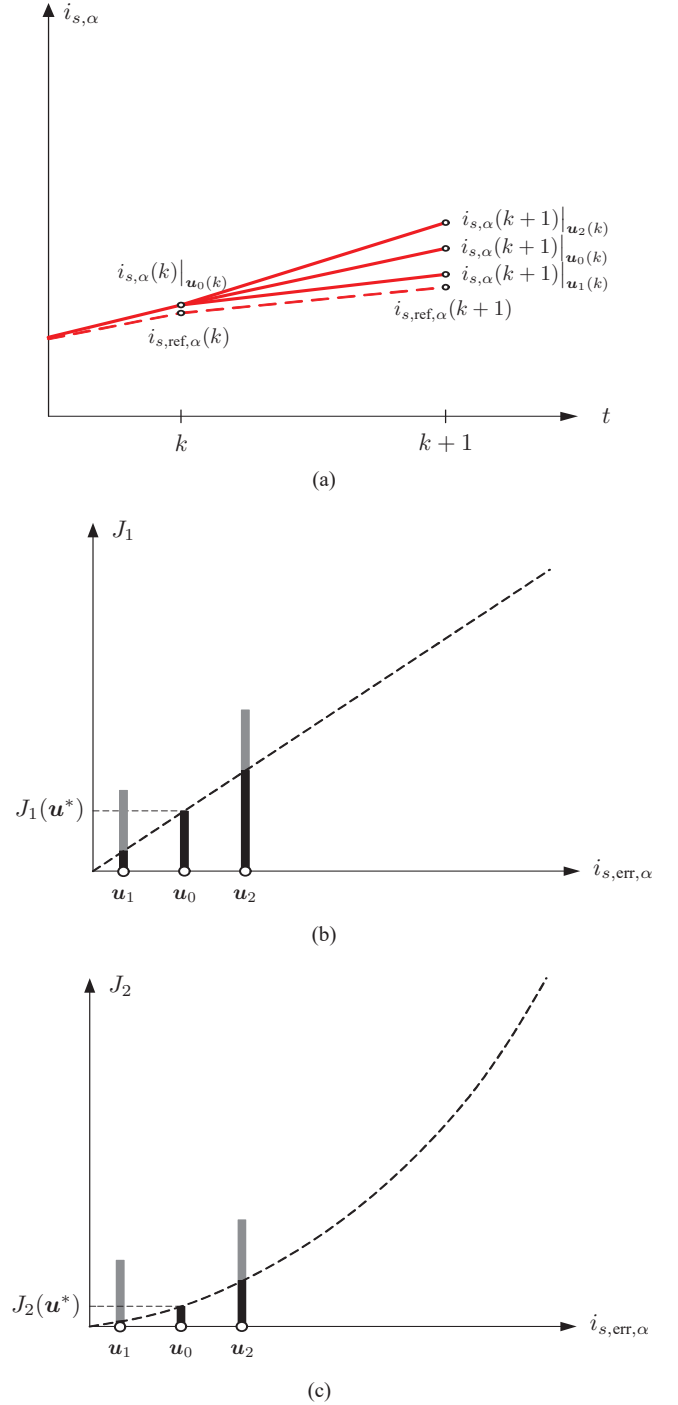
Fig. 5. Impact of the choice of norm on the selection of the switch position when the current error is small. (a) Instance of the problem. (b) Penalization of the current error and the switching effort based on the \ell_1 -norm. (c) Penalization of the current error and the switching effort based on the (squared) \ell_2 -norm. The switching cost is shown with the gray bar and the tracking error with the black bar.
