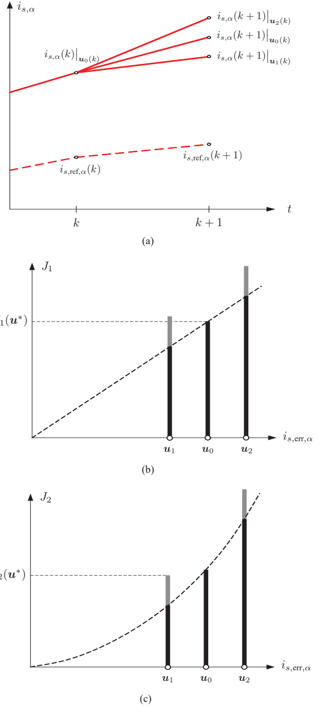
Fig. 6. Impact of the choice of norm on the selection of the switch position when the current error is large. (a) Instance of the problem. (b) Penalization of the current error and the switching effort based on the \ell_1 -norm. (c) Penalization of the current error and the switching effort based on the (squared) \ell_2 -norm. The switching cost is shown with the gray bar and the tracking error with the black bar.
