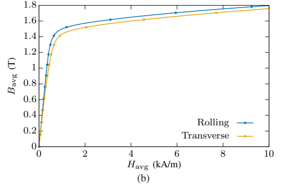
Fig. 2. Anhyseretic magnetization in the rolling and transverse directions of the NO silicon steel sheet. The anhyseretic curves are extracted from the measured major BH loops. (a) Logarithmic plot. (b) Linear plot for H_{\text{avg}} \leq 10 kA/m.
