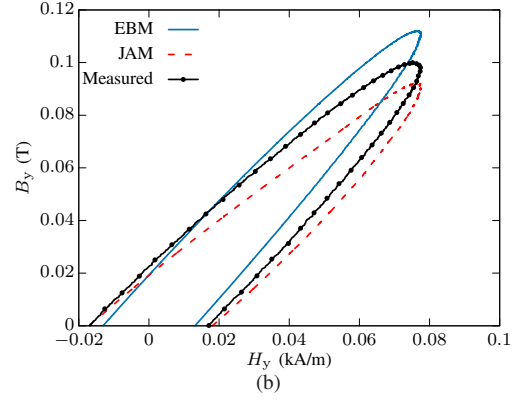
Fig. 11. Results for rotational low field excitation |\mathbf{B}| = 0.1 T. (a) H_x B_x -loci (b) H_y B_y -loci.
