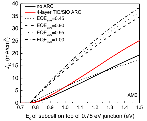
Fig. 2. Projected J_{sc} at AM0 for a 0.78 eV subcell in a multijunction architecture where incident light is filtered by an optically thick subcell. In addition, upper limits for J_{sc} for 0.78 eV subcell with different average EQEs are shown.
